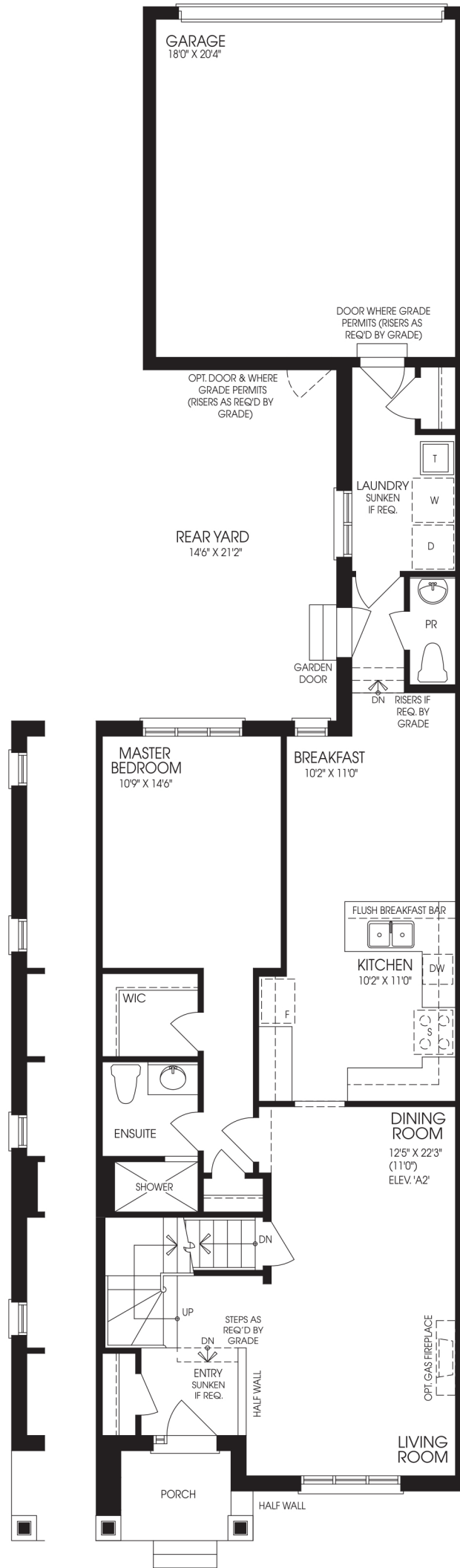
END UNIT MAIN FLOOR ELEVATION 'A2'
